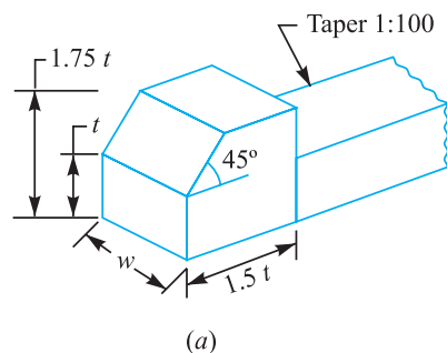
Fig. 13.2. Gib-head key.
