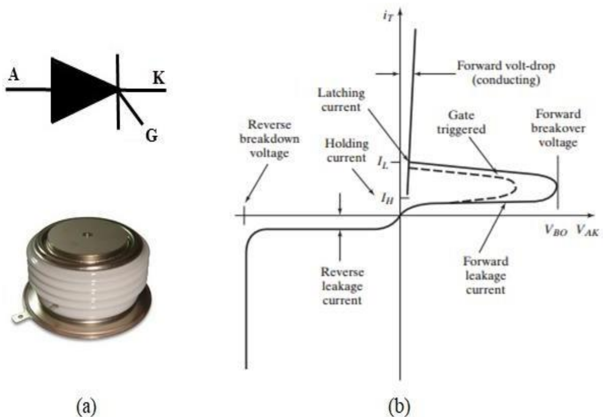
Figure 1.4: (a) SCR symbol, and (b) Practical characteristics.
