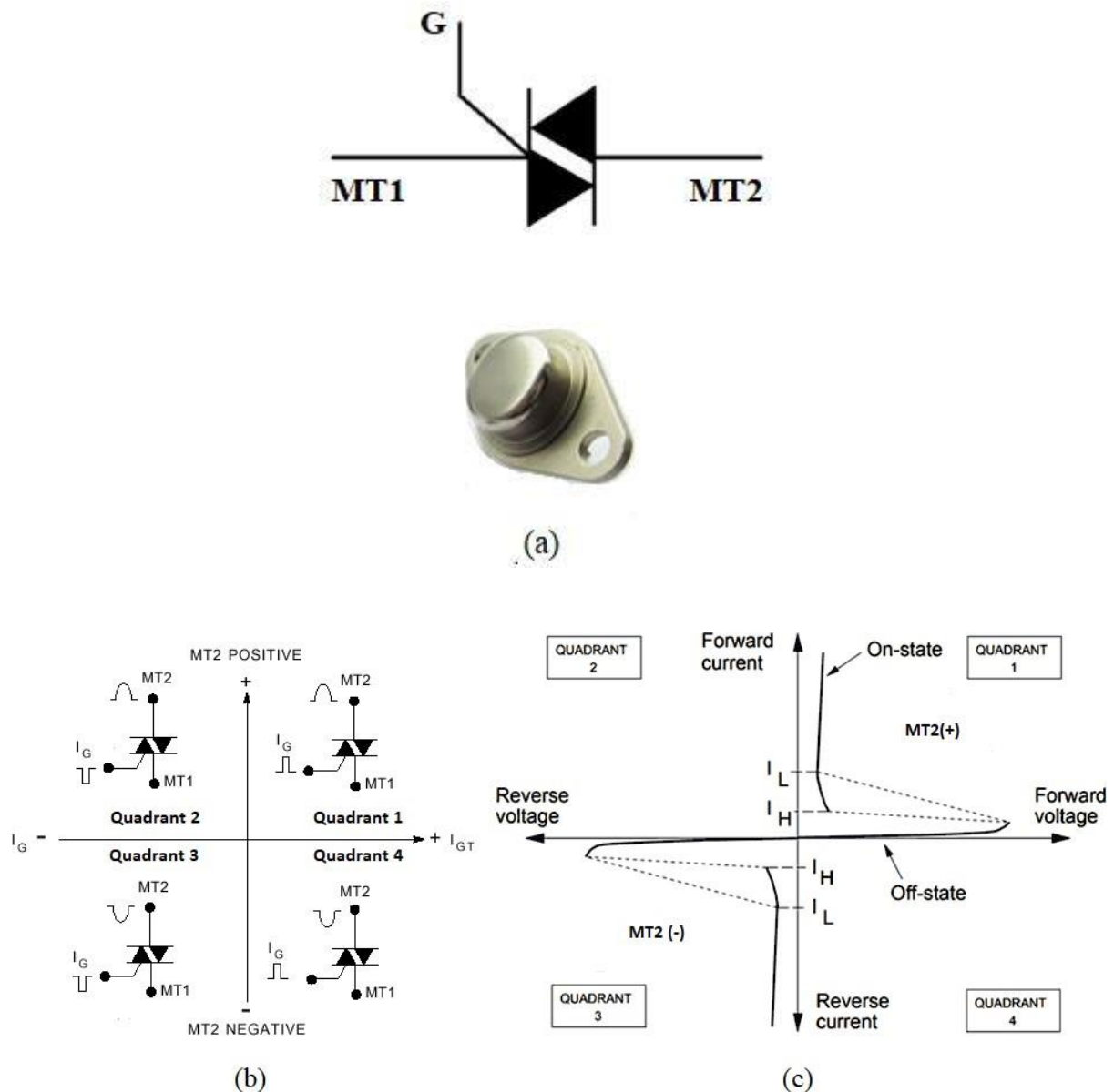
Figure 1.5: (a) TRIAC symbol, (b) Quadrant diagram, and (c) Practical characteristics.
