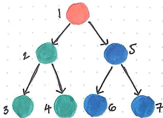
Depth-first search
