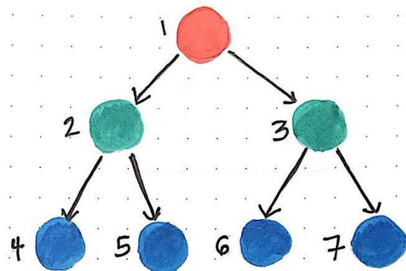
Breadth-first search
