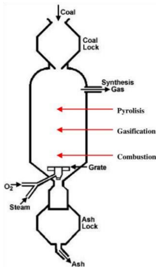
Fig.1 : Coal gasifier
