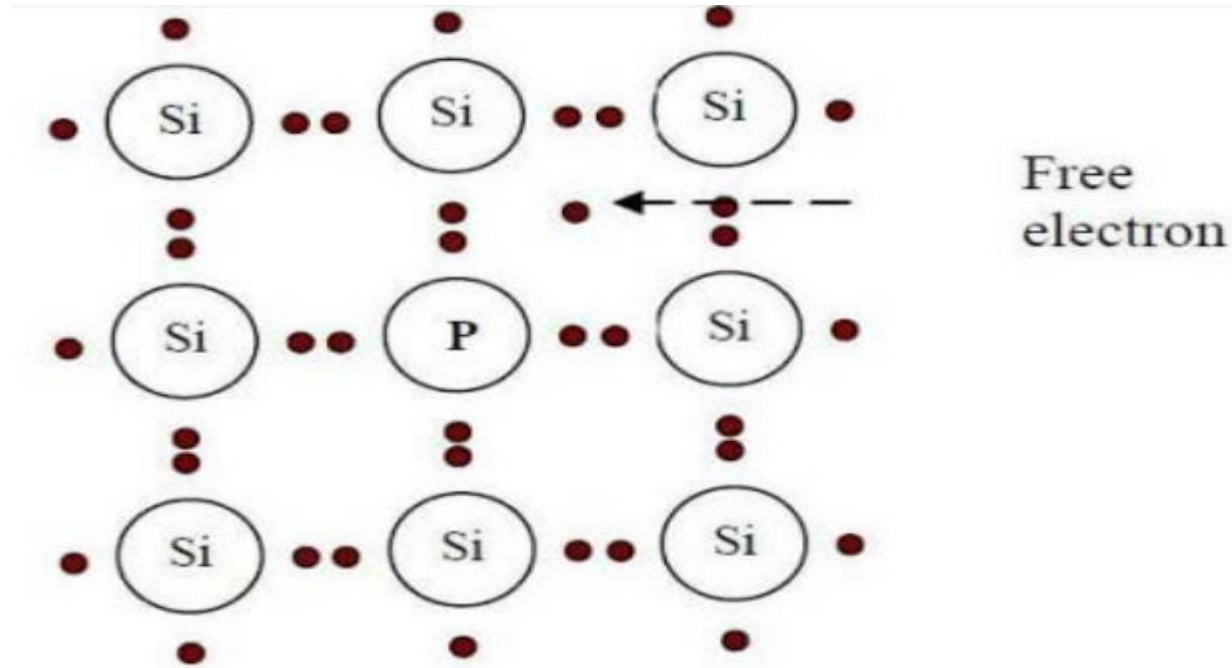
Fig 2. N-Type Semiconductor
