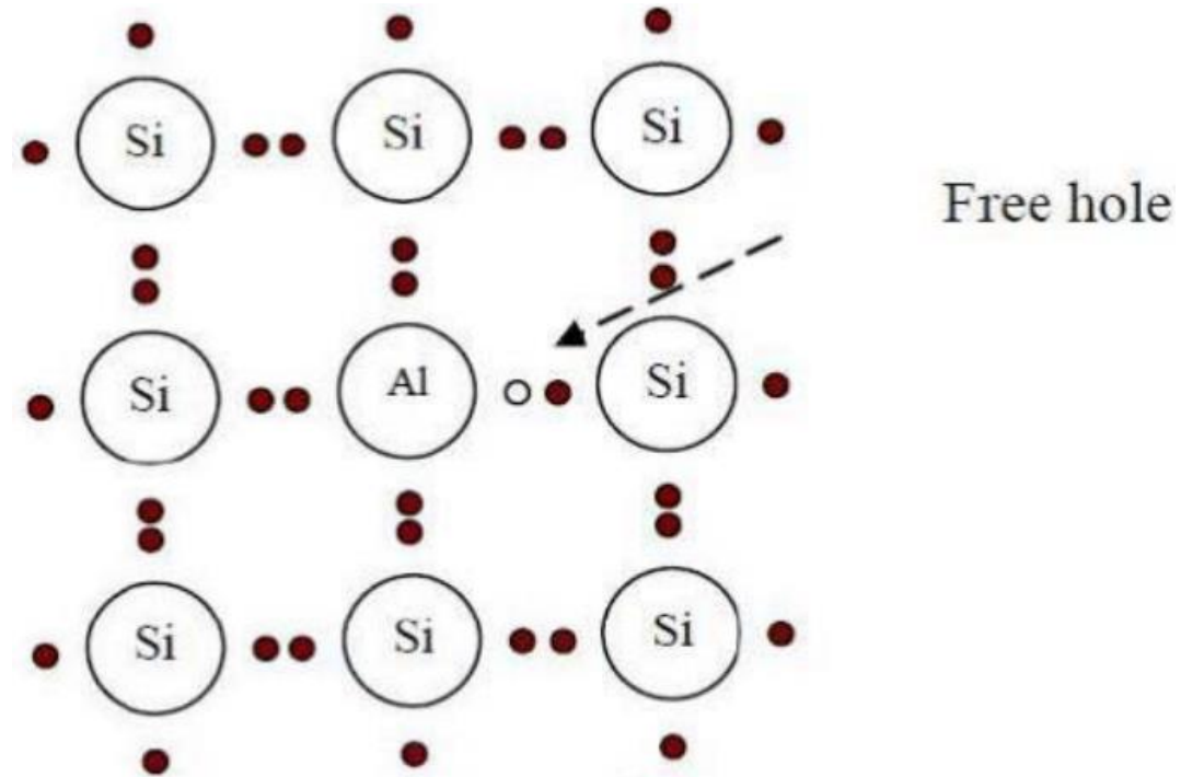
Fig 3. p-Type Semiconductor
