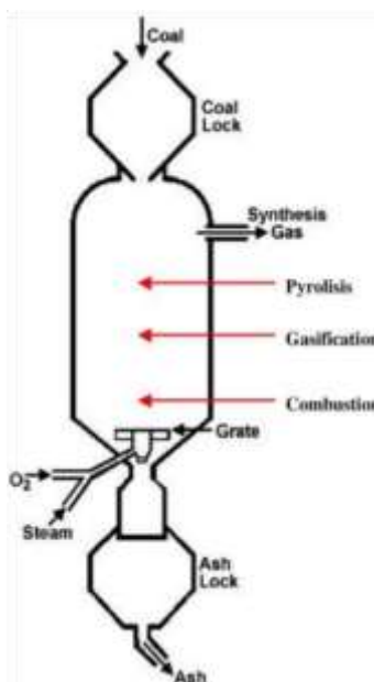
Fig.1: Coal gasifier
