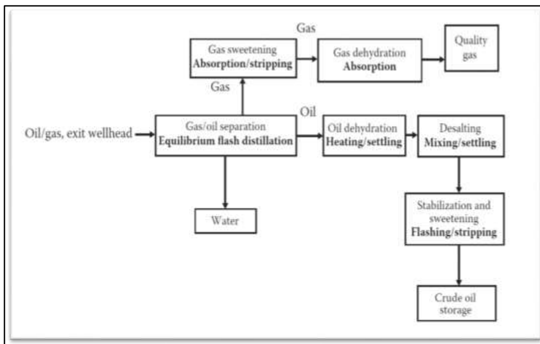
Figure 5.2. Pre-treatment unit of crude oil and gas.
