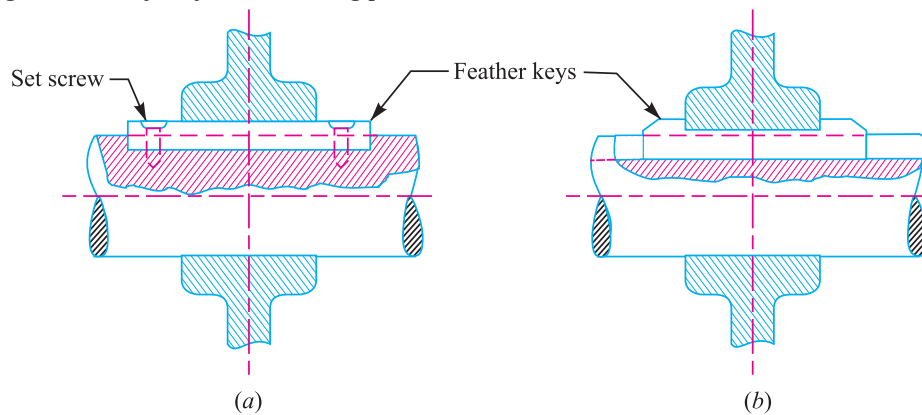
Fig. 13.3. Feather key.
