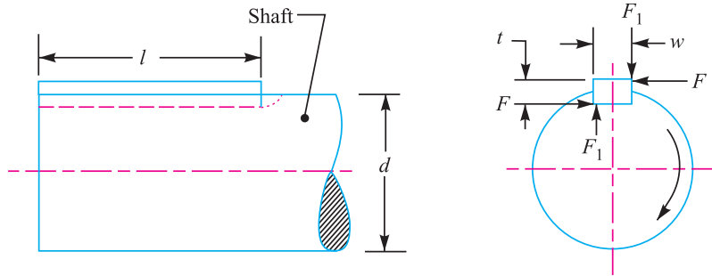
Fig. 13.9. Forces acting on a sunk key.
