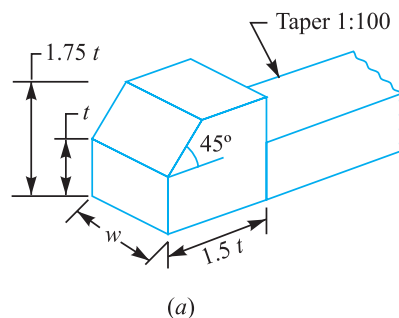
Fig. 13.2. Gib-head key.
