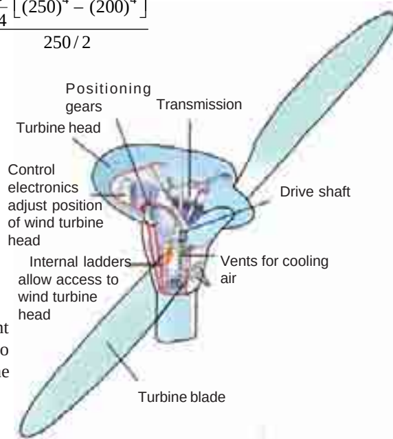
Wind turbine.
