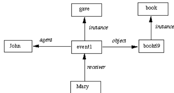
Fig. A Semantic Network for a Sentence
