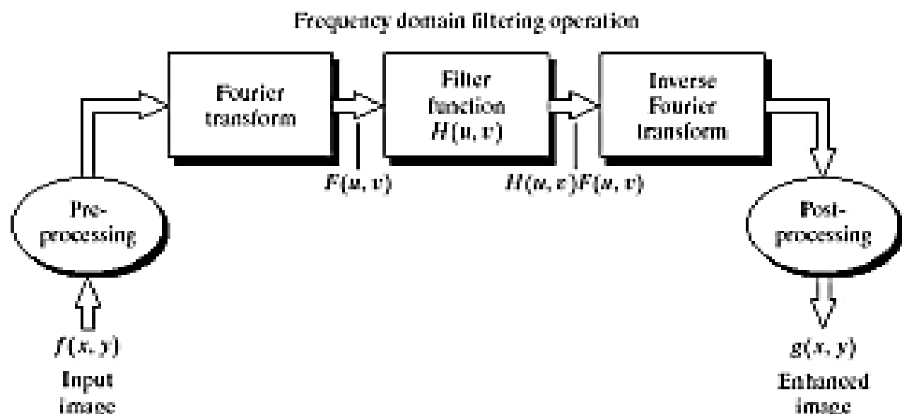
Figure 7.3 Basic steps for filtering in the frequency domain
