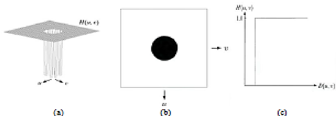
Figure 8.11 (a) IHPF transfer function. (b) IHPF as an image. (c) IHPF radial cross section
