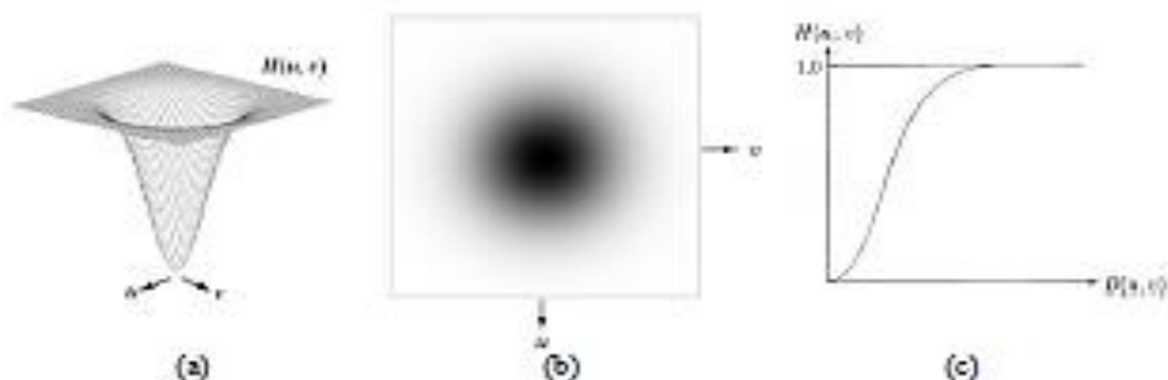
Figure 8.15 (a) GHPF transfer function. (b) GHPF as an image. (c) GHPF radial cross section
