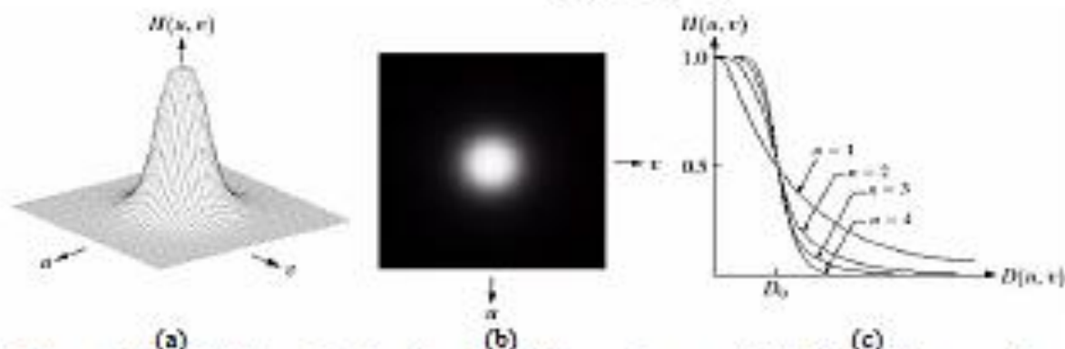
Figure 8.4 (a) BLPF transfer function. (b) BLPF as an image. (c) BLPF radial cross section
