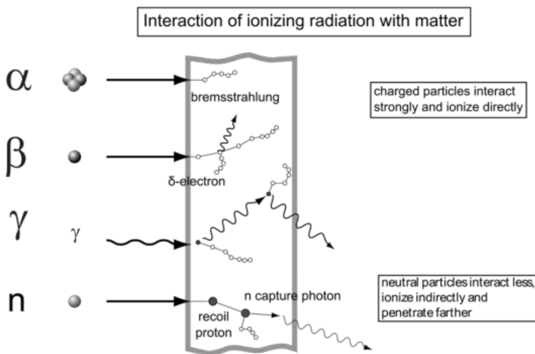
Interaction of ionizing radiation with matter
