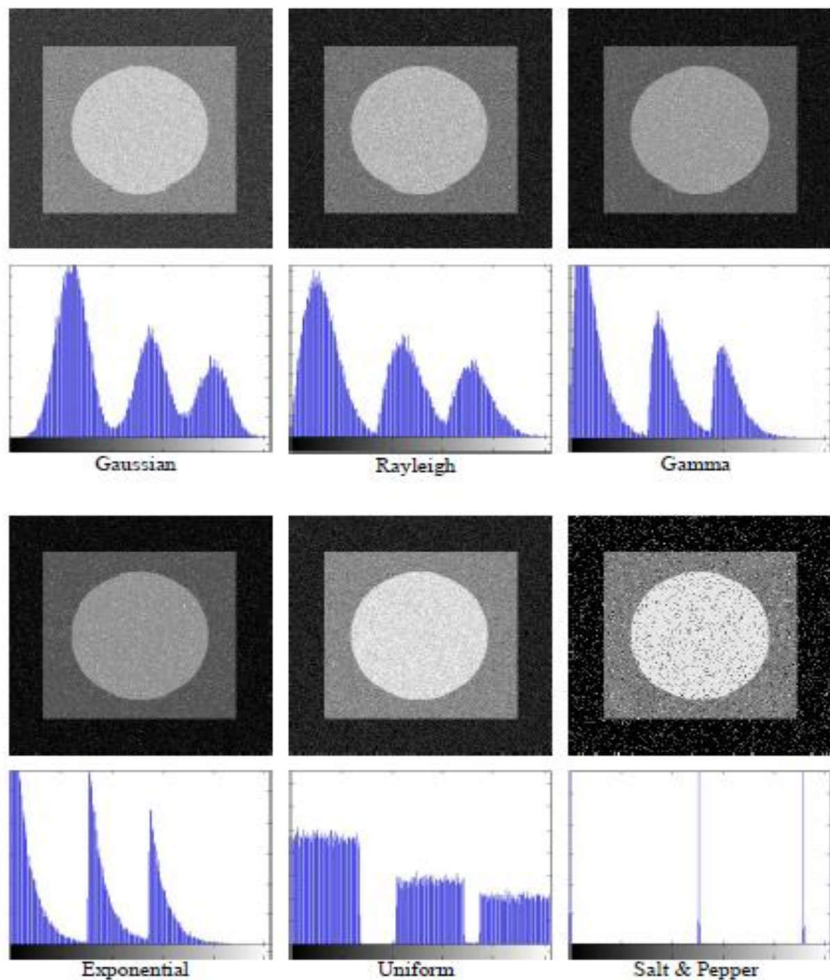
Figure 10.6 Images and histograms from adding Gaussian, Rayleigh, Gamma, Exponential, Uniform, and Salt & Pepper noise.
