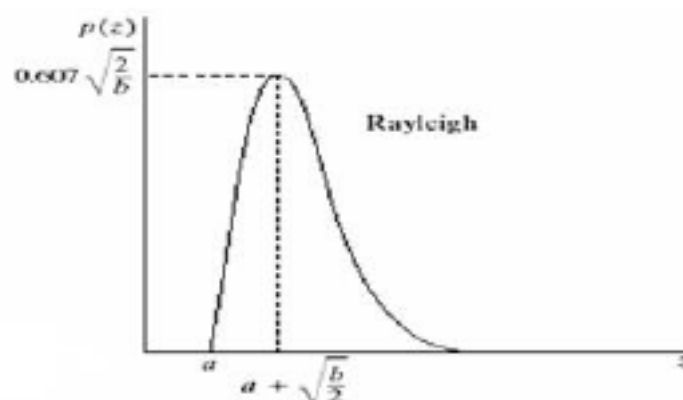
Figure 10.3 Rayleigh noise PDF
