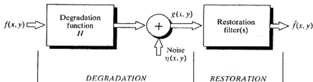
Figure 10.1 A model of the image degradation/restoration process
