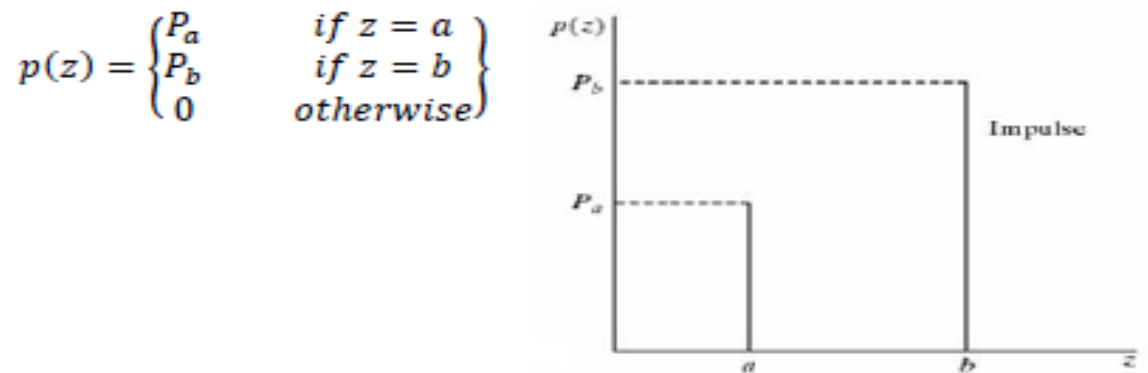
Figure 10.4 Impulse noise PDF
