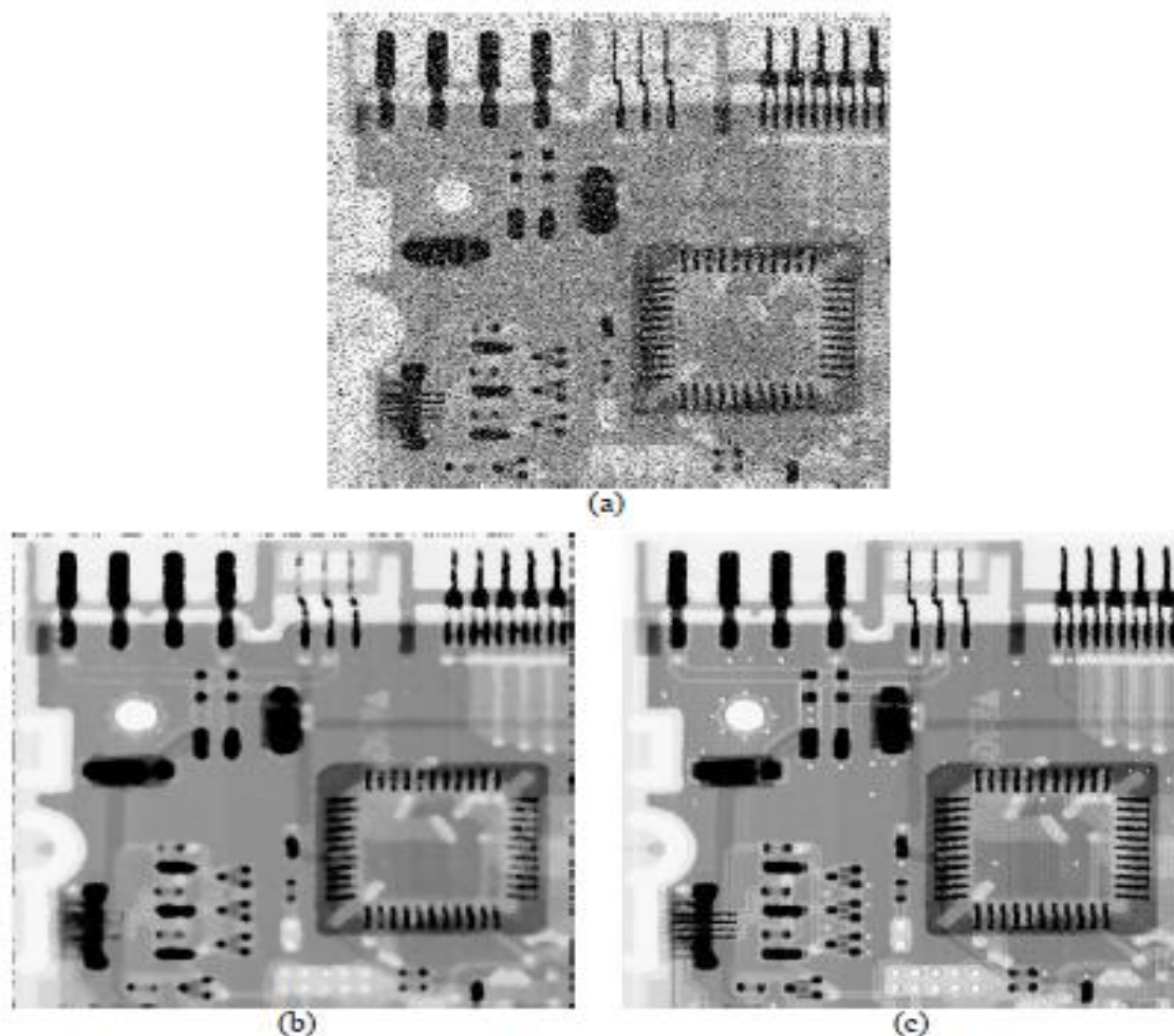
Figure 10.10 (a) Image corrupted by salt&pepper noise with density 0.25. (b) Result obtained using a 7 \times 7 median filter. (c) Result obtained using adaptive median filter with S_{\max} = 7 .
