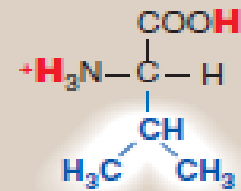
Valine
