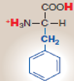
Phenylalanine
