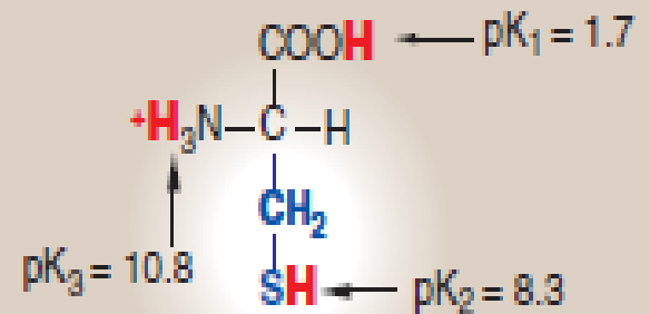
Cysteine
