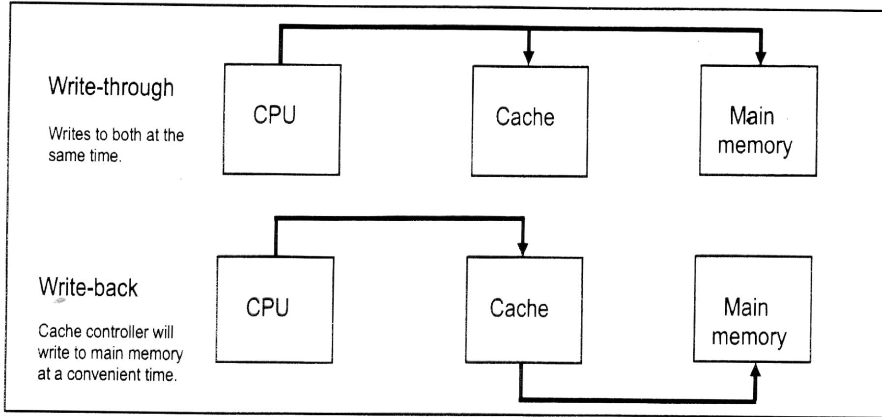
Figure 22-9. Methods of Updating Main Memory
