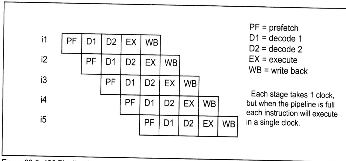
Figure 23-3. 486 Pipeline Stages
