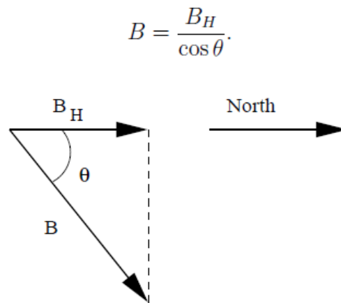
Figure (1): The relationship between the earth's magnetic field B and the horizontal component B_H at the earth's surface in the northern hemisphere.
