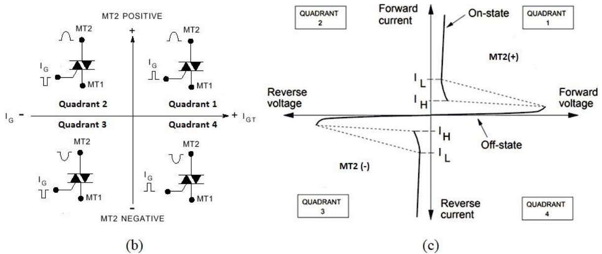
Figure 1.5: (a) TRIAC symbol, (b) Quadrant diagram, and (c) Practical characteristics.
