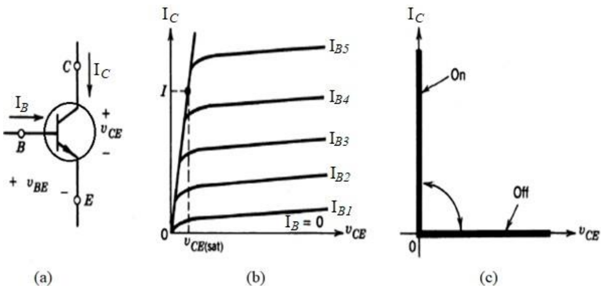
Figure 1.7: (a) BJT symbol, (b) practical characteristics of BJT, and (c) idealized characteristics of BJT.
