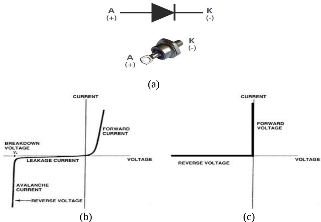
Figure 1.3: (a) Diode symbol, (b) Practical characteristics, and (c) Ideal characteristics.
