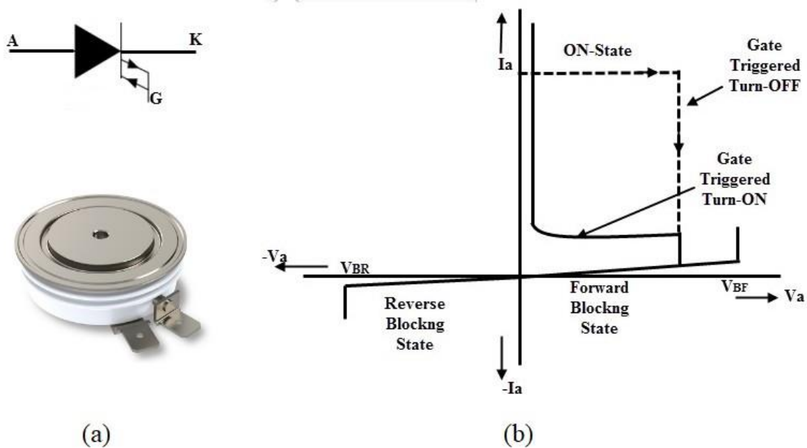
Figure 1.6: (a) GTO symbol, and (b) Practical characteristics.
