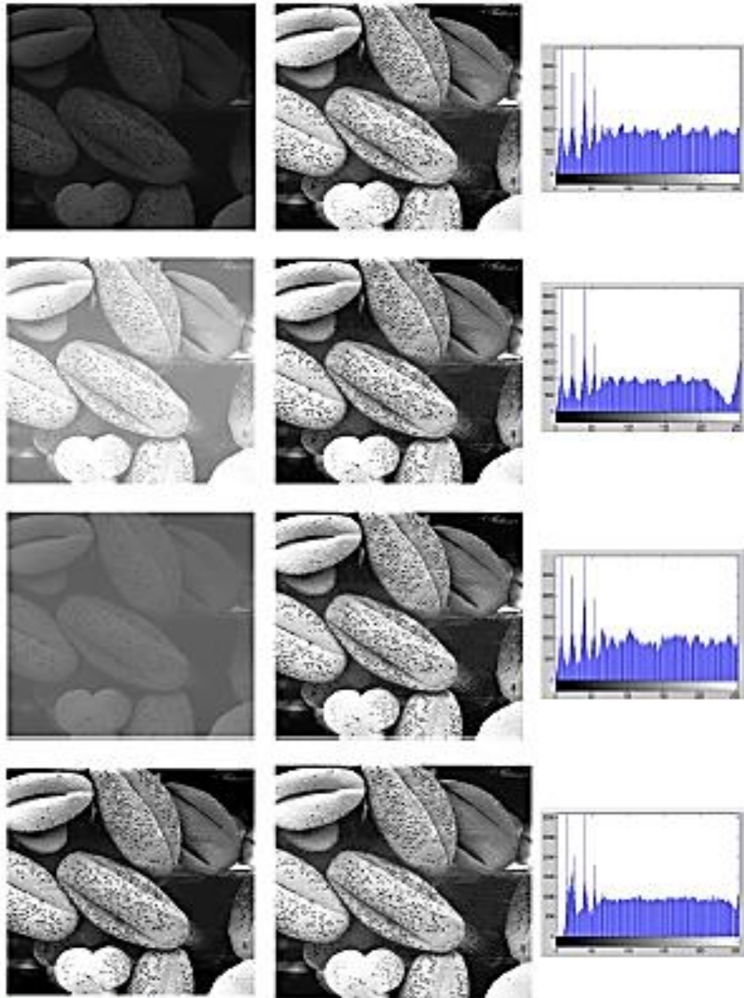
Figure 5.8 Left column original images. Center column corresponding histogram equalized images. Right column histograms of the images in the center column.
