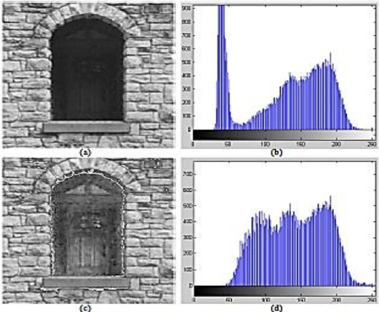
Figure 5.3 Contrast stretching. (a) Original image. (b) Histogram of (a). (c) Result of contrast stretching. (d) Histogram of (c).
