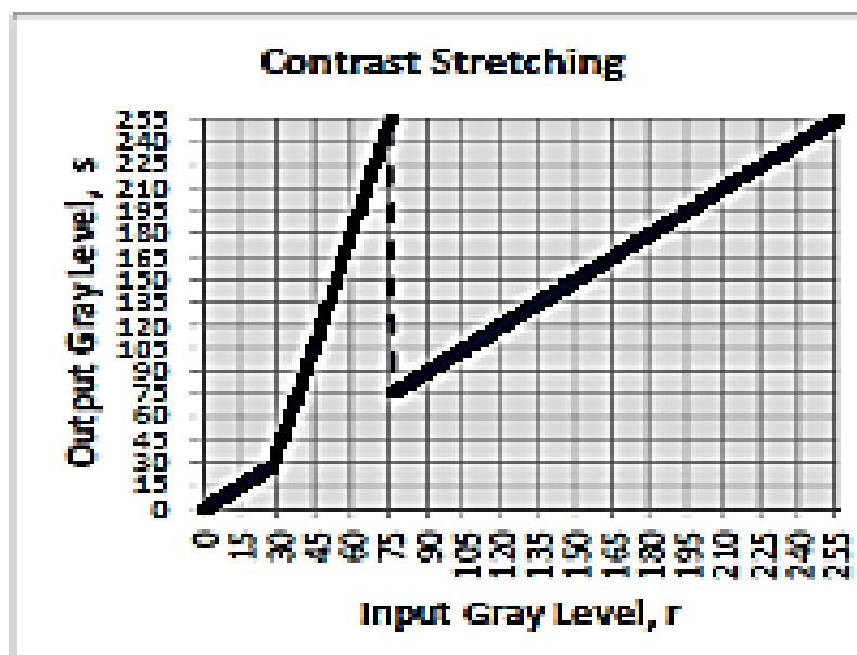
Figure 3.2 Plot of above piecewise linear function
