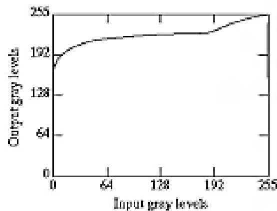
Figure 5.11 HE transformation function of Figure 5.10(a)
