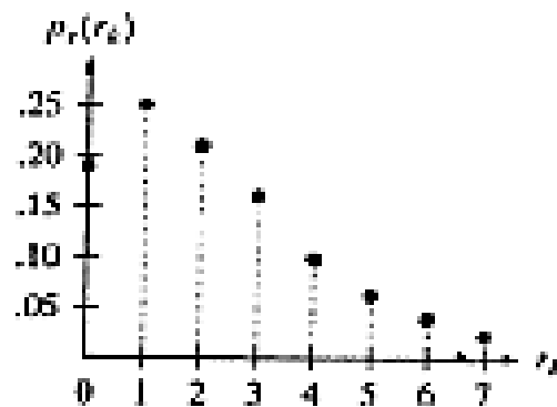
Normalized histogram
