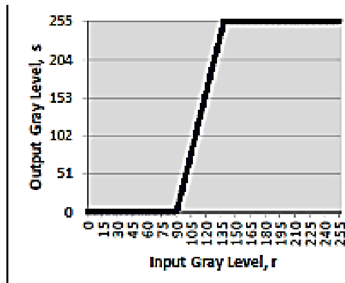
Figure 5.4 Full contrast-stretching
