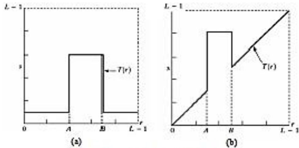
Figure 5.6 Gray-level slicing
