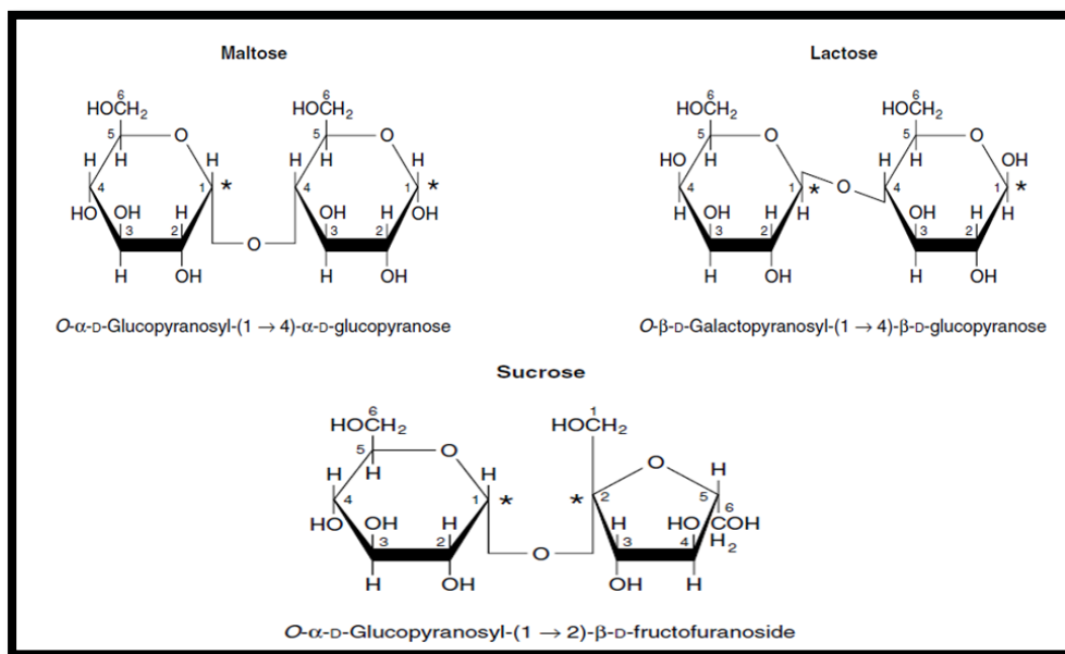
Structures of important disaccharides
