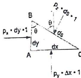
Fig.( 2.1 ) Forces on a fluid element .
