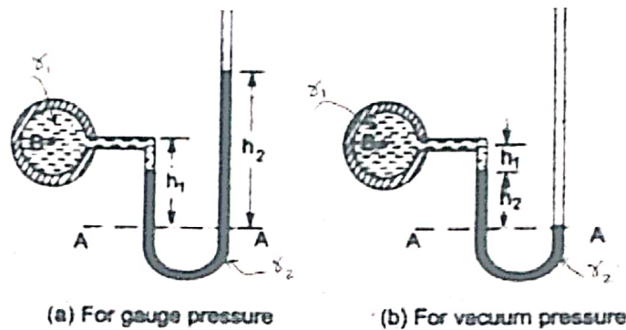
Fig.( 2.5 ) U- tube Manometer.
