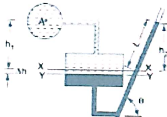
Fig.(2.8) Inclined manometer
