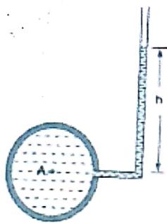
Fig.(2.4) Piezometer.
