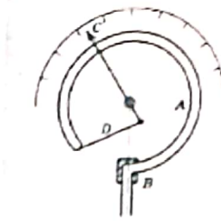
Fig.(2.11) Schematically shown of Bourdon gage
