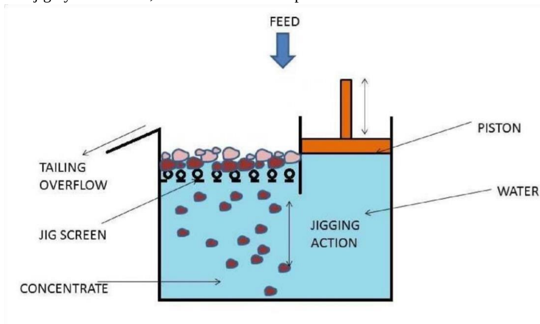
Figure 2.2 Conceptual diagram illustrates the basic principles of a jig
