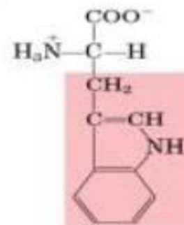
Tryptophan
