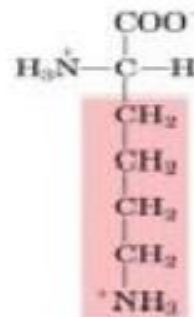
Lysine
