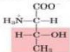
Threonine
