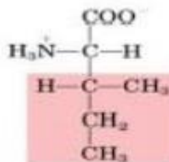
Isoleucine
