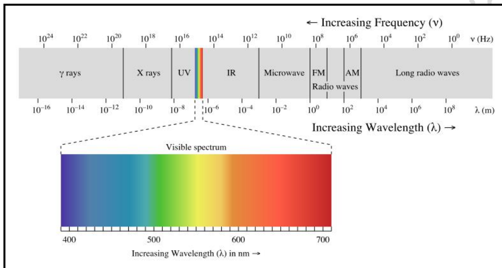
Figure 1: Electromagnetic Spectrum
