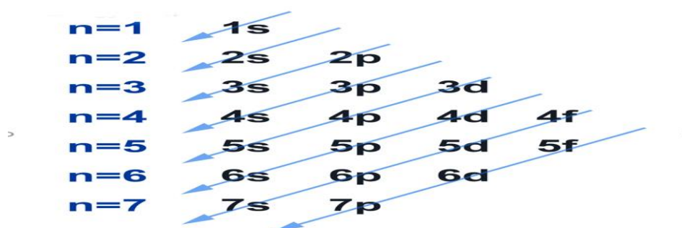
Figure 1: arrangement of the secondary energy levels(orbitals). Orbital (1S) is filled first with electrons then 2S then 2P then 3S then 3P then 4S then 3d and so far:
