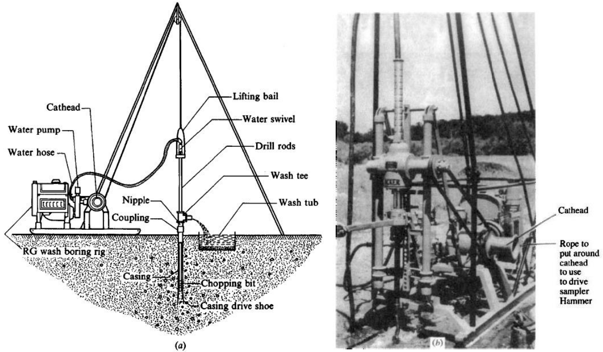
Figure 3-2 (a) Schematic of wash-boring operations; (b) photograph of wash-boring operation. Note weight in lower right foreground to advance casing and to take penetration numbers when the chopping bit is replaced with the split spoon. (The Acker Drill Company.)
