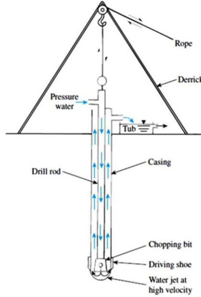
Figure 3.2 Wash boring
