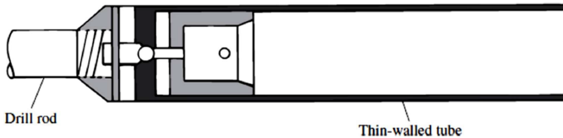
Fig. 3-6 Thin-walled tube
