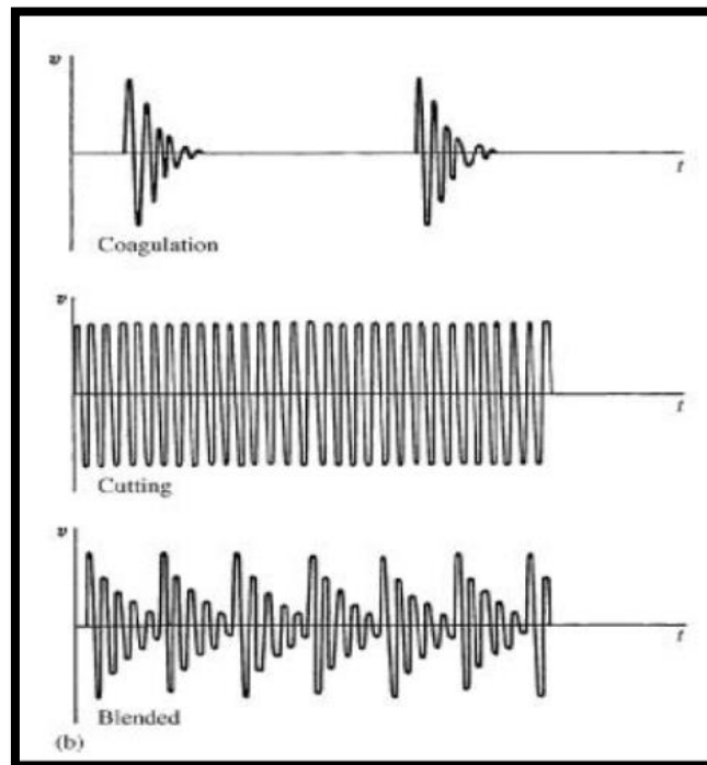
Figure 1 (a) Block diagram for an electrosurgical unit. High-power, high-frequency oscillating currents are generated and coupled to electrodes to incise and coagulate tissue, (b) Three different electric voltage waveforms available at the output of electrosurgical units for carrying out different functions
