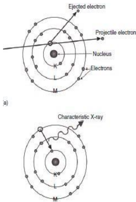
Figure 3 (a) An atom being ionised when a K – shell electron is ejected by an energetic projectile electron. (b) The vacancy in the K -shell, resulting from ionization of the atom, is filled by an M -shell electron. A characteristic X -ray is given off.
