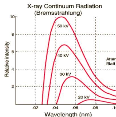
Figure (2) bremmstrahlung radiation
