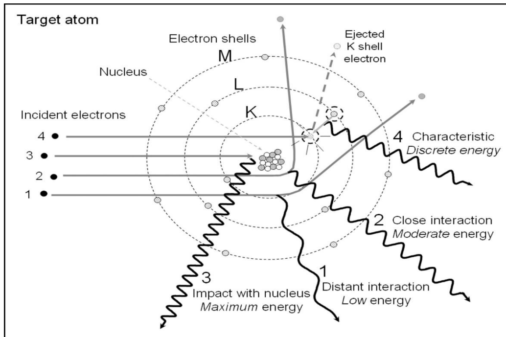
Figure4: X-ray production by energy conversion. Events 1, 2, and 3 depict incident electrons interacting in the vicinity of the target nucleus, resulting in bremsstrahlung production caused by the deceleration and change of momentum, with the emission of a continuous energy spectrum of x-ray photons. Event 4 demonstrates characteristic radiation emission, where an incident electron with energy greater than the K-shell binding energy collides with and ejects the inner electron creating an unstable vacancy. An outer shell electron transitions to the inner shell and emits an x-ray with energy equal to the difference in binding energies of the outer electron shell and K shell that are “characteristic” of tungsten.
