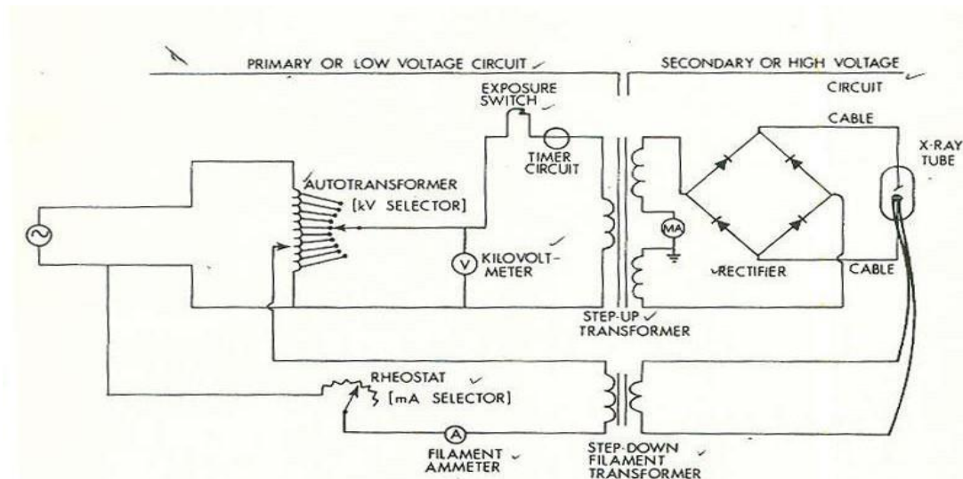
Figure 14.12. Simplified wiring of a single phase x-ray unit, with full-wave rectification.
