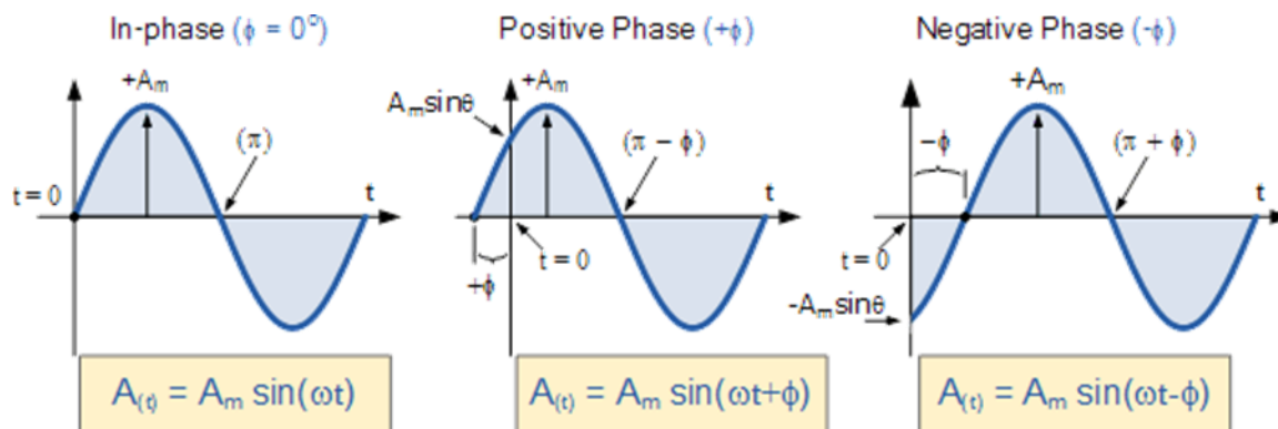
Figure 4. Phase Relationship
