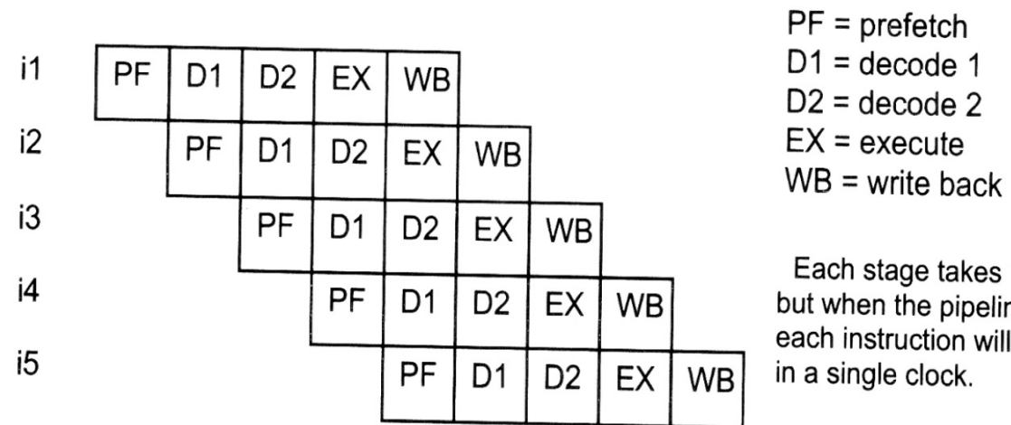
Figure 23-3. 486 Pipeline Stages
