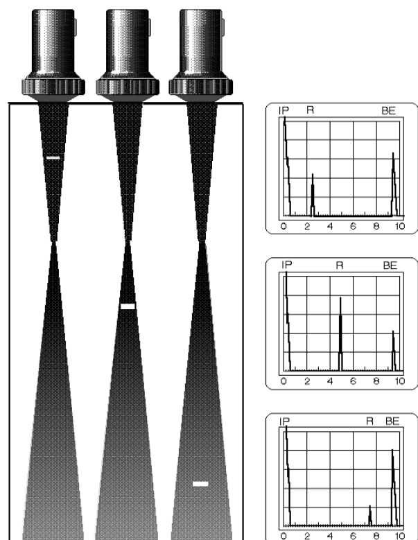
Fig. 60 Reflectors at different depths and their echoes
