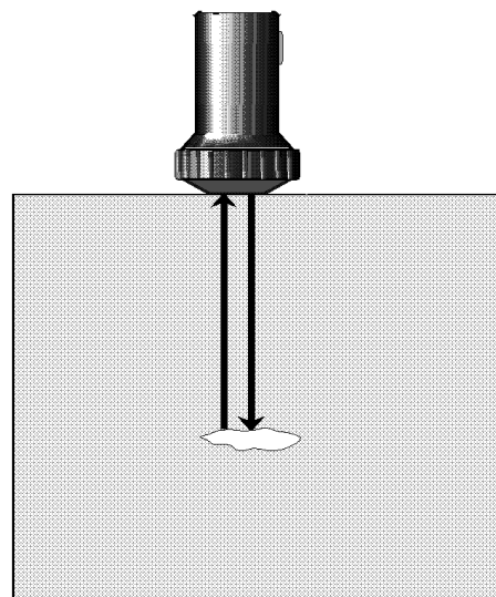
Fig. 2a Plane flaw – straight-beam probe
