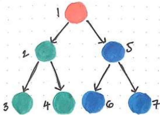
Depth-first search
