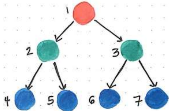
Breadth-first search
