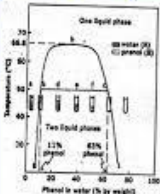
Temperature-composition diagram for the binary two phase region of water and phenol
