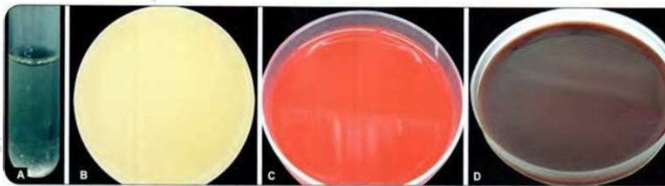
Figure (1): A. Peptone water; B. Nutrient agar; C. Blood agar; D. Chocolate agar.
