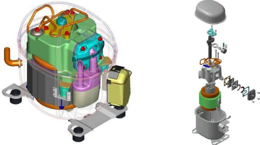
Figure 2 hermetic compressor
