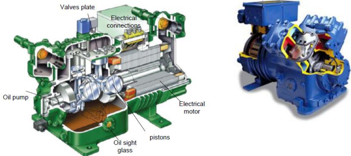
Figure 3 semi-hermetic compressor
