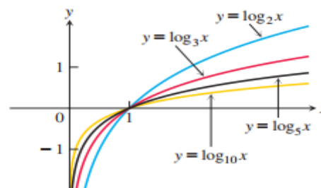
Figure 4 Graphs of four logarithmic functions
