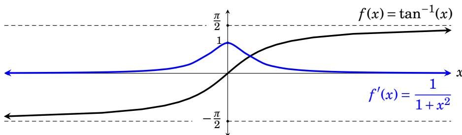
Figure 25.3. The function \tan^{-1}(x) and its derivative \frac{1}{1+x^2} . Note \lim_{x \rightarrow \infty} \frac{1}{1+x^2} = 0 and \lim_{x \rightarrow -\infty} \frac{1}{1+x^2} = 0 , reflecting the fact that the tangent lines to y = \tan^{-1}(x) become closer and closer to horizontal as x \rightarrow \pm\infty . The derivative bumps up to 1 at x = 0 , where the tangent to y = \tan^{-1}(x) is steepest, with slope 1
