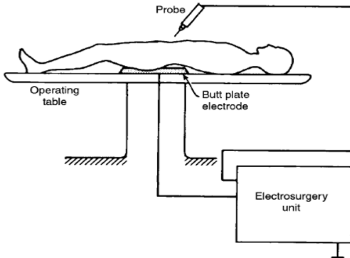
Figure 4. The basic arrangement of the electrosurgical unit.
