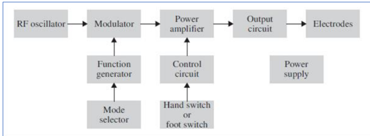
Figure 3. The block diagram of a typical electrosurgical unit.
