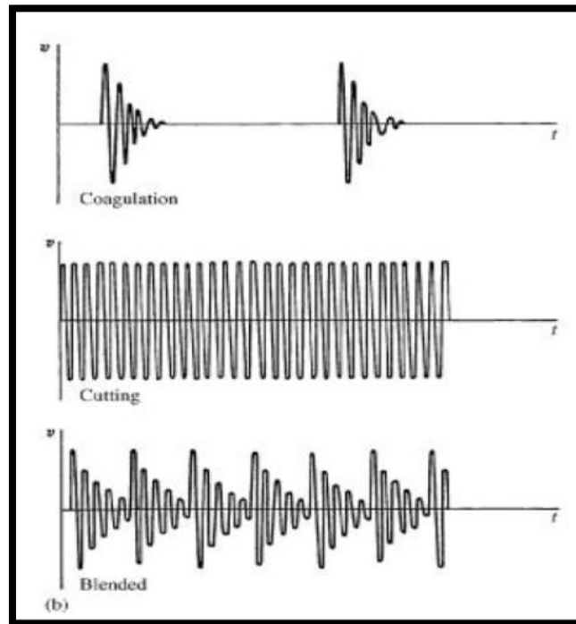
Figure 1 (a) Block diagram for an electro-surgical unit. High-power, high-frequency oscillating currents are generated and coupled to electrodes to incise and coagulate tissue, (b) Three different electric voltage waveforms available at the output of electro-surgical units for carrying out different functions
