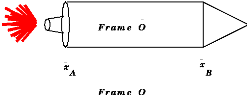
Figure 7.8: Length contraction
