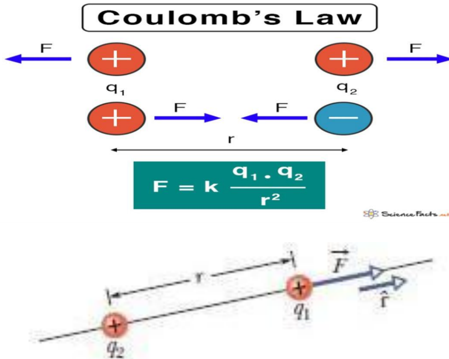
Figure 2: The electrostatic force on particle 1 can be described in terms of a unit vector along an axis through the two particles, radially away from particle 2.
