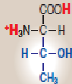
Threonine
