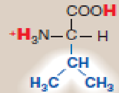
Valine
