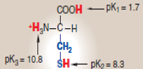
Cysteine
