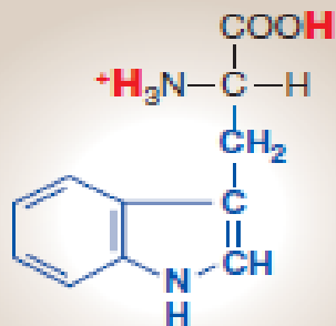
Tryptophan
