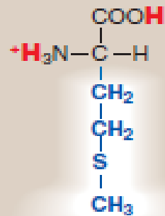
Methionine
