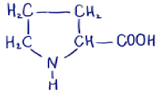
Proline
