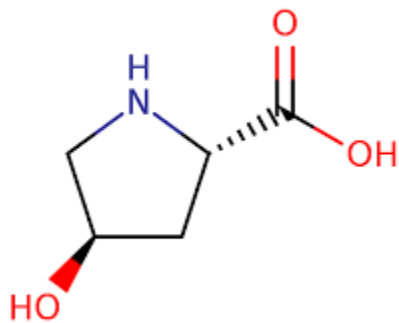
4-hydroxyproline
