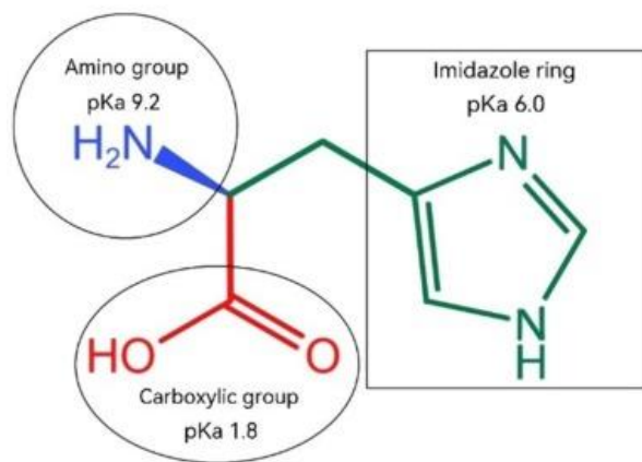
Histidine
