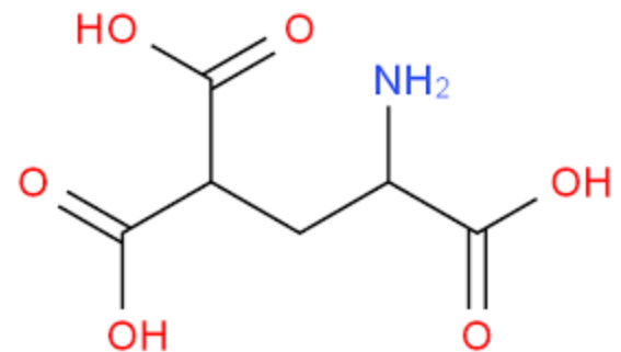
Gamma-carboxy-L-glutamic acid
