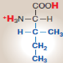
Isoleucine
