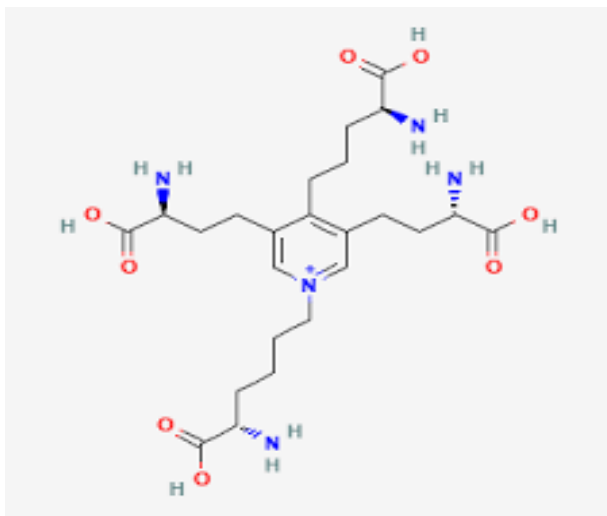
Desmosine,
