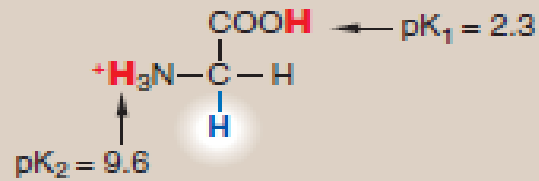
Glycine
