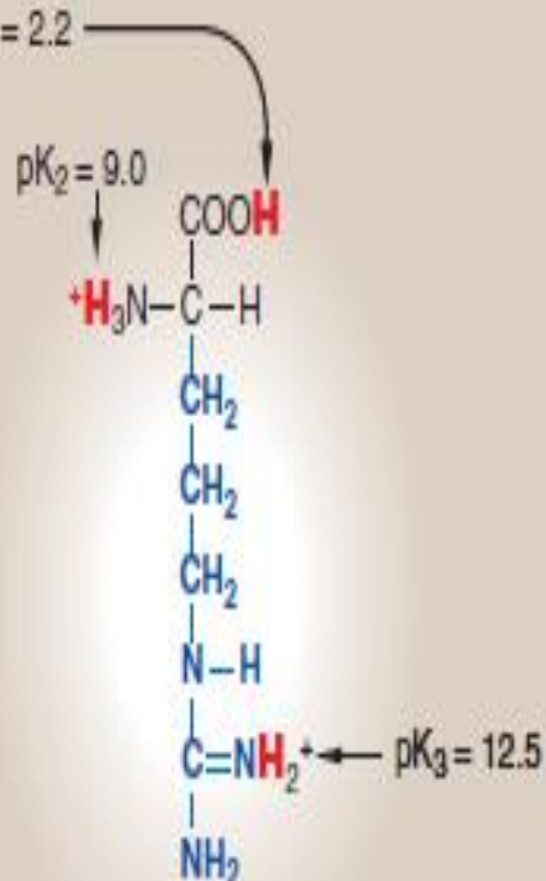
Arginine
