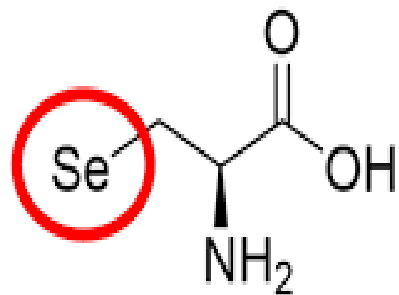
Selenocysteine
