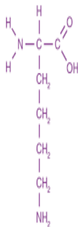
Lysine
