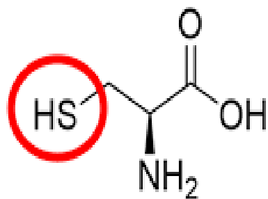
Cysteine
