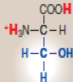
Serine
