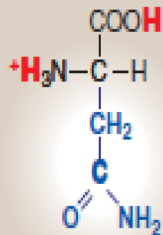
Serine
